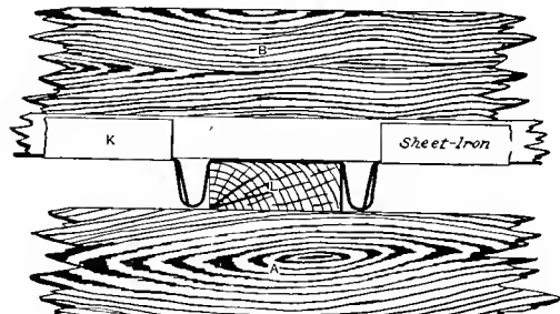
Fig. 2383. Longitudinal Section of Ridge-pole.
